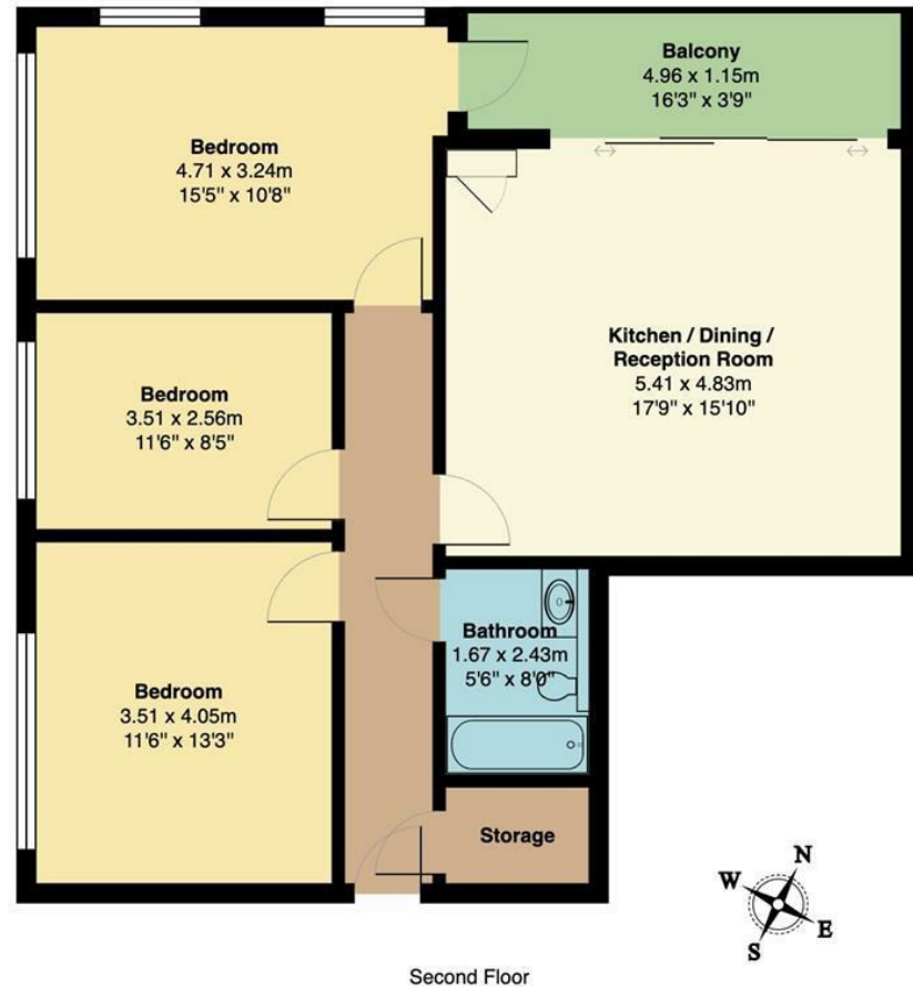
Second Floor
