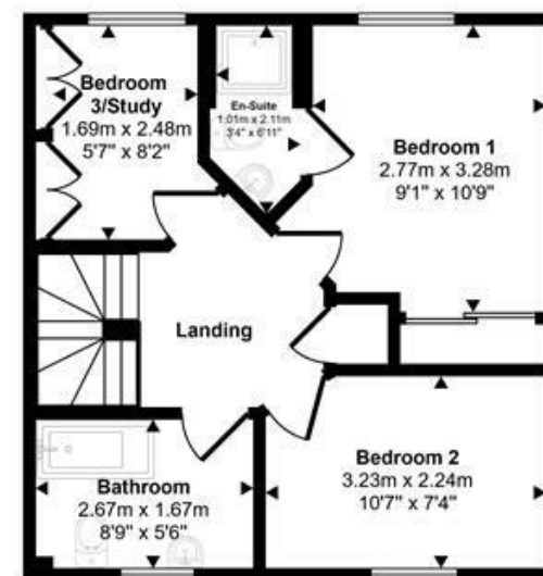
First Floor Approx 38 sq m / 409 sq ft
