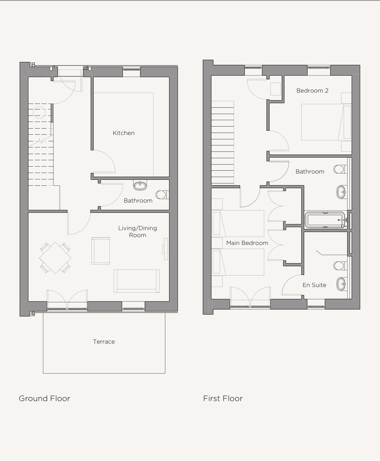
EXAMPLE TWO BEDROOM, COTTAGE FLOOR PLAN
